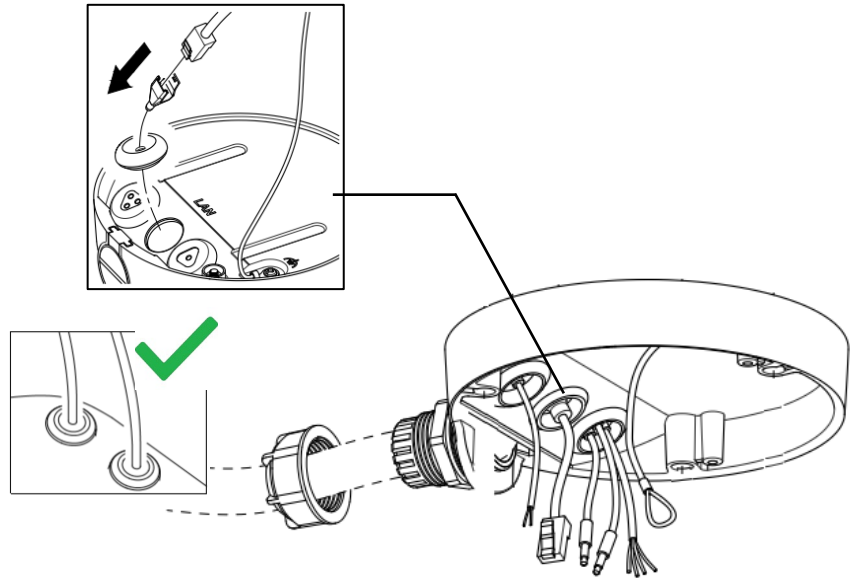
Figure 2 Cabling
