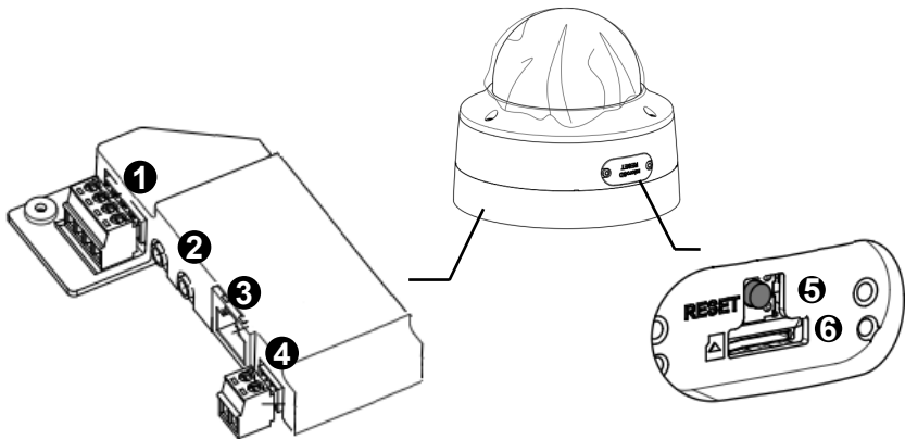
Figure 1 Camera Connectors
